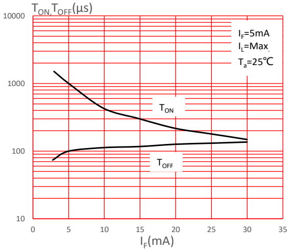
FIG.7: T_{ON}, T_{OFF} vs. LED Forward Current
